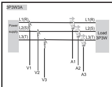
Orientation of Clamp sensor
